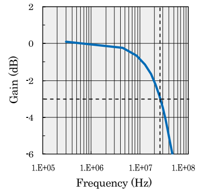
Fig6. Frequency Response
